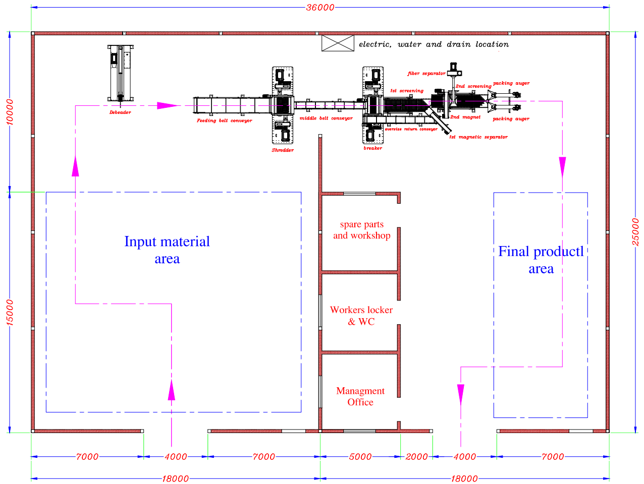
plant layout for tire recycling line 500 kg/hr
